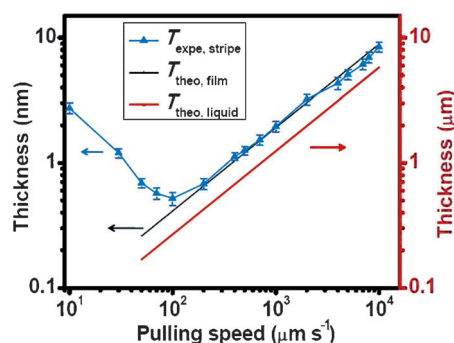
Figure 3. Plots of T_{\text{expe, stripe}} , T_{\text{theo, liquid}} and T_{\text{theo, film}} versus the pulling speed. T_{\text{expe, stripe}} is the experimental thickness (average value) of microstripes. T_{\text{theo, liquid}} is the theoretical thickness of entrained liquid film ( T_{\text{theo, liquid}} \cdot T_{\text{theo, film}} is the theoretical thickness of solute film after solvent evaporation).
